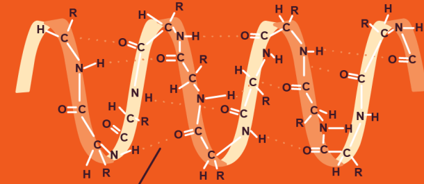
\alpha helix
