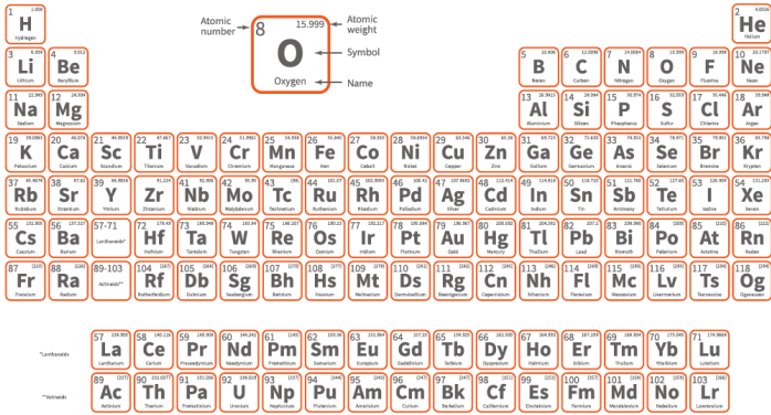
Figure 2. The periodic table of elements.
