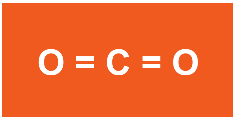
Figure 8. Carbon dioxide is a linear, nonpolar molecule
