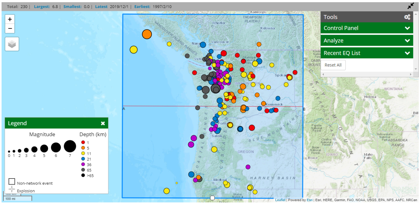
( https://pressbooks.bccampus.ca/geoglabmanualv2/wp-content/uploads/sites/1032/2020/08/Figure-16.3-Epicentres-notable-PNW.png )
