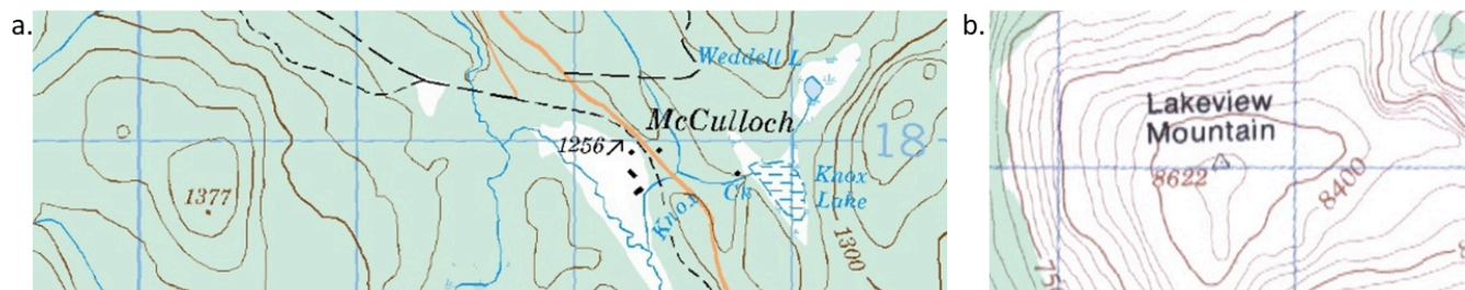
Figure 15.6. a. Example of a spot height (elevation = 1377) and a benchmark (elevation = 1256). b. Example of a horizontal control point (elevation = 8622). Note: Elevation units may be feet or metres – you need to check the map. Sources: a. NTS 1:50,000 map sheet 82E14 ( http://ftp.geogratis.gc.ca/pub/nrcan_rncan/raster/topographic/50k/082/e/14/ ) (Kelowna) 4th edition. b. NTS 1:50,000 map sheet 92H01 ( http://ftp.geogratis.gc.ca/pub/nrcan_rncan/raster/topographic/50k/092/h/01/ ) (Ashnola River) 2nd edition. Natural Resources Canada, Open Government License-Canada ( https://open.canada.ca/en/open-government-licence-canada ).
