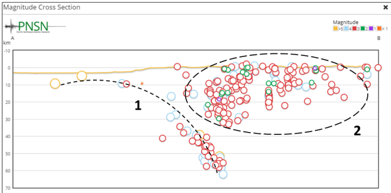
Figure 18.4. Cross section (A to B in Figure 18.3) showing depth and magnitude of notable earthquakes within the shaded area in Figure 18.3 (open circles). The solid yellow line shows the ground surface relative to sea level (0 m). Two separate groups of earthquakes are identified by the dashed black lines and labelled 1 and 2. You will identify the difference between the groups in EX3. Source: Adapted by C. Welch, with data from the Pacific Northwest Seismic Network Notable Events ( https://pnsn.org/earthquakes/notable ). Used with permission. [Image description]
