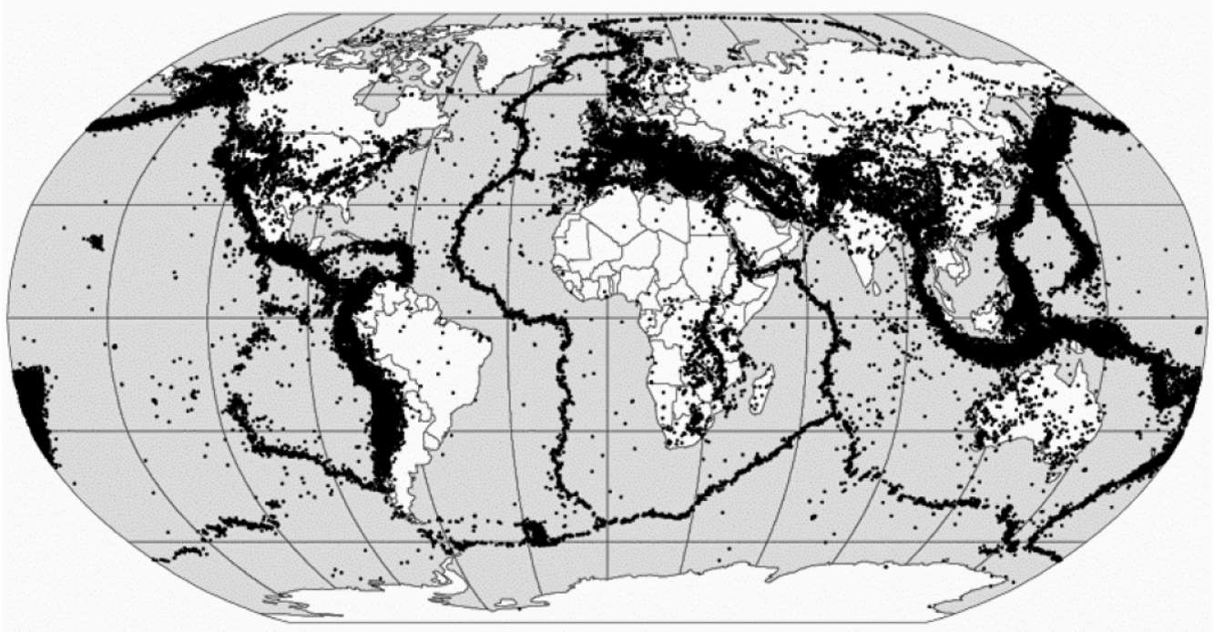
( https://pressbooks.bccampus.ca/geoglabmanualv2/wp-content/uploads/sites/1032/2020/08/figure-16.2-earthquake-epicentres.png )
