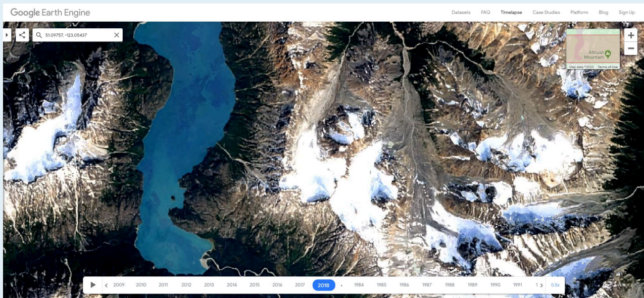
( https://pressbooks.bccampus.ca/geoglabmanualv2/wp-content/uploads/sites/1340/2021/03/Figure-20.6-Huscroft-2018-imagery.jpg )
