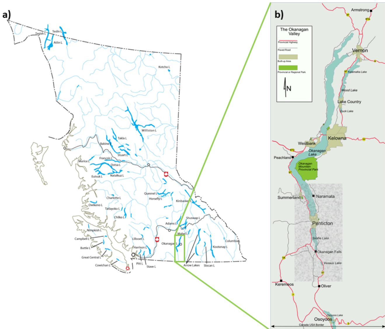
( https://pressbooks.bccampus.ca/geoglabmanualv2/wp-content/uploads/sites/1340/2020/07/figure-22.1.png )
