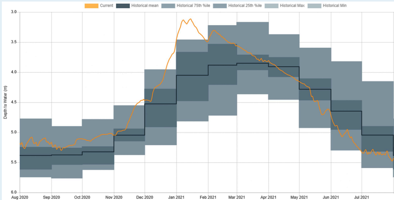
Figure 20.4. Example of groundwater level annual summary graph for Observation well #353. Source: Groundwater levels at BC Obs Well 353 © BC Water Tool ( https://www.bcwatertool.ca/ ) contains groundwater level data licensed under the Environment Canada ( https://www.canada.ca/en/transparency/terms.html ) / Water Survey of Canada ( https://wateroffice.ec.gc.ca/disclaimer_info_e.html ).
