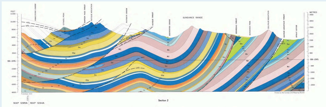
Figure 17.8. Geological Survey of Canada: Banff East-Half Cross Section. Source: Geological Survey of Canada ( https://geoscan.nrcan.gc.ca/starweb/geoscan/servlet.starweb?path=geoscan/fulle.web&search1=R=108961 ), Open Government License.
