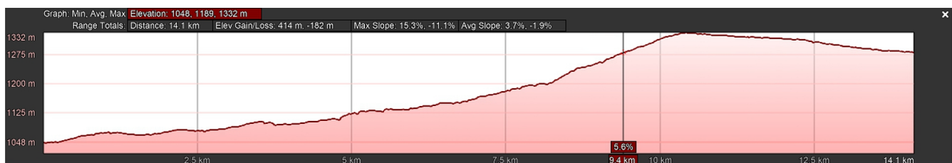
Figure 15.10. Topographic profile of the length of the Trans Canada Highway shown in Figure 15.5. Source: Google Earth, used in accordance with Google Earth Guidelines ( https://www.google.com/permissions/geoguidelines/ ).
