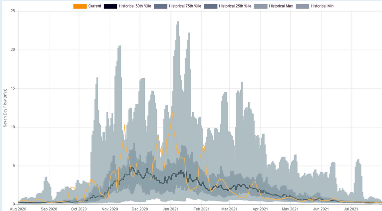
Figure 20.3. Example of stream hydrograph from the Nicomekl River hydrograph 08MH155 station. Source: Stream discharge in Nicomekl River at Station 08MH155 © BC Water Tool ( https://www.bcwatertool.ca/ ) contains stream discharge data licensed under Environment Canada ( https://www.canada.ca/en/transparency/terms.html ) / Water Survey of Canada ( https://wateroffice.ec.gc.ca/disclaimer_info_e.html ).
