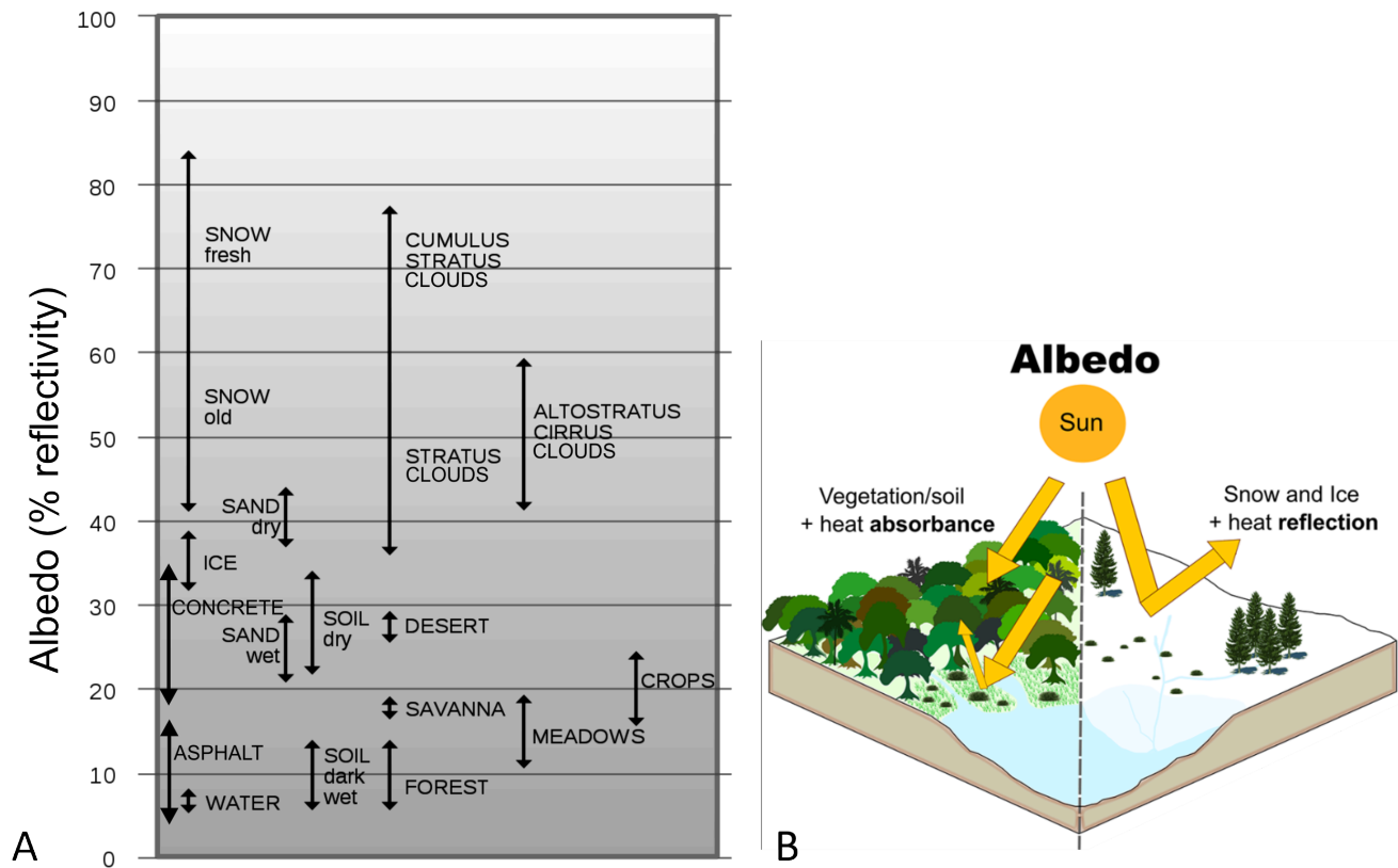
Figure 2.6. Albedo of common surfaces. Source: H. Grobe (2000) ( https://commons.wikimedia.org/wiki/File:Albedo-e_hg.png )CC BY-SA 2.5. B: Pictorial demonstration of how albedo controls reflection and absorption of energy received from the sun. Source: Prevedello et al (2019) ( https://journals.plos.org/plosone/article?id=10.1371/journal.pone.0213368 ). CC BY. [Image description]
