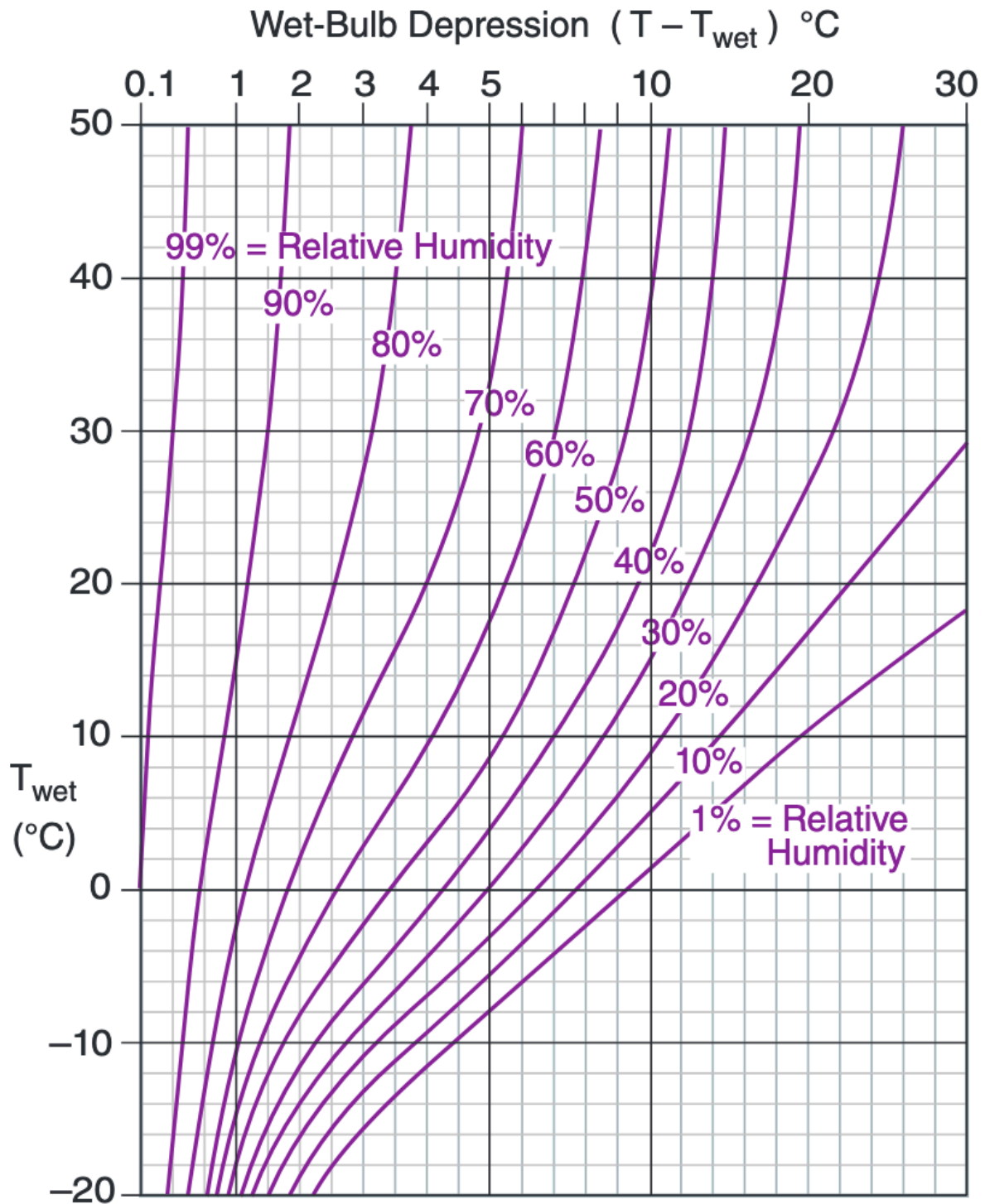
Figure 8.6. Psychrometric graph, to find relative humidity from wet and dry-bulb temperatures. Source: R. Stull (2017) [PDF] ( https://www.eoas.ubc.ca/books/Practical_Meteorology/prmet102/Ch04-watervapor-v102b.pdf ) CC BY-NC-SA.
