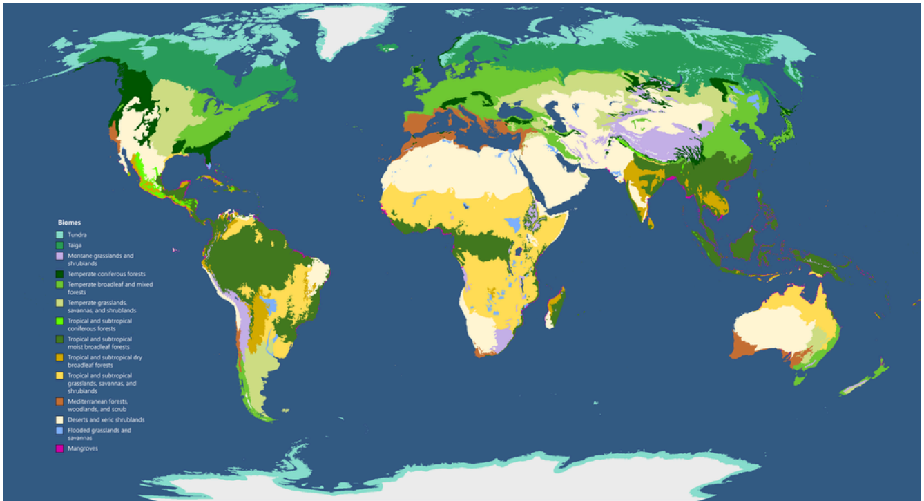
( https://pressbooks.bccampus.ca/geoglabmanualv2/wp-content/uploads/sites/1340/2021/06/figure-1-lab-11.png )
