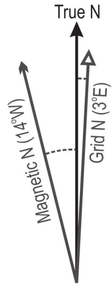
Figure 15.2. A declination diagram. In this case, Magnetic N is 14^\circ west of True N, and Grid N is 3^\circ east of True N. Source: I. Saunders, CC BY-NC-SA 4.0.
