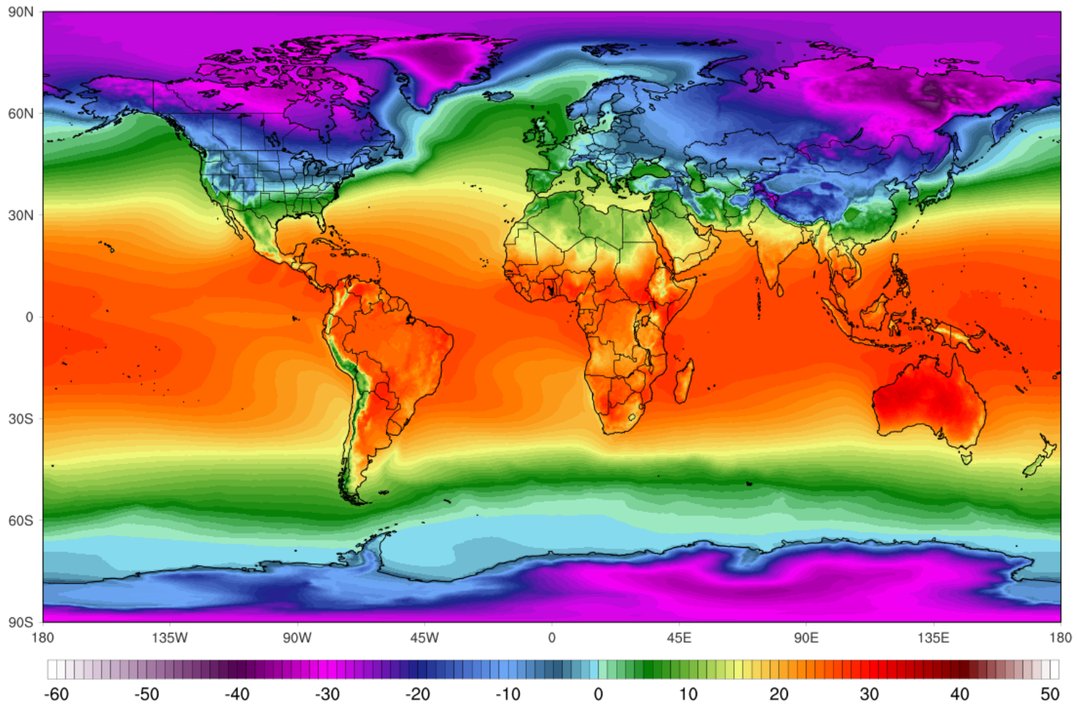
Figure 2.3. Average January air temperature at 2 meters above the Earth's surface, 1951-2020 (data – ECMWF European Reanalysis V5). Image Source: Courtesy of Climatereanalyzer.org .
