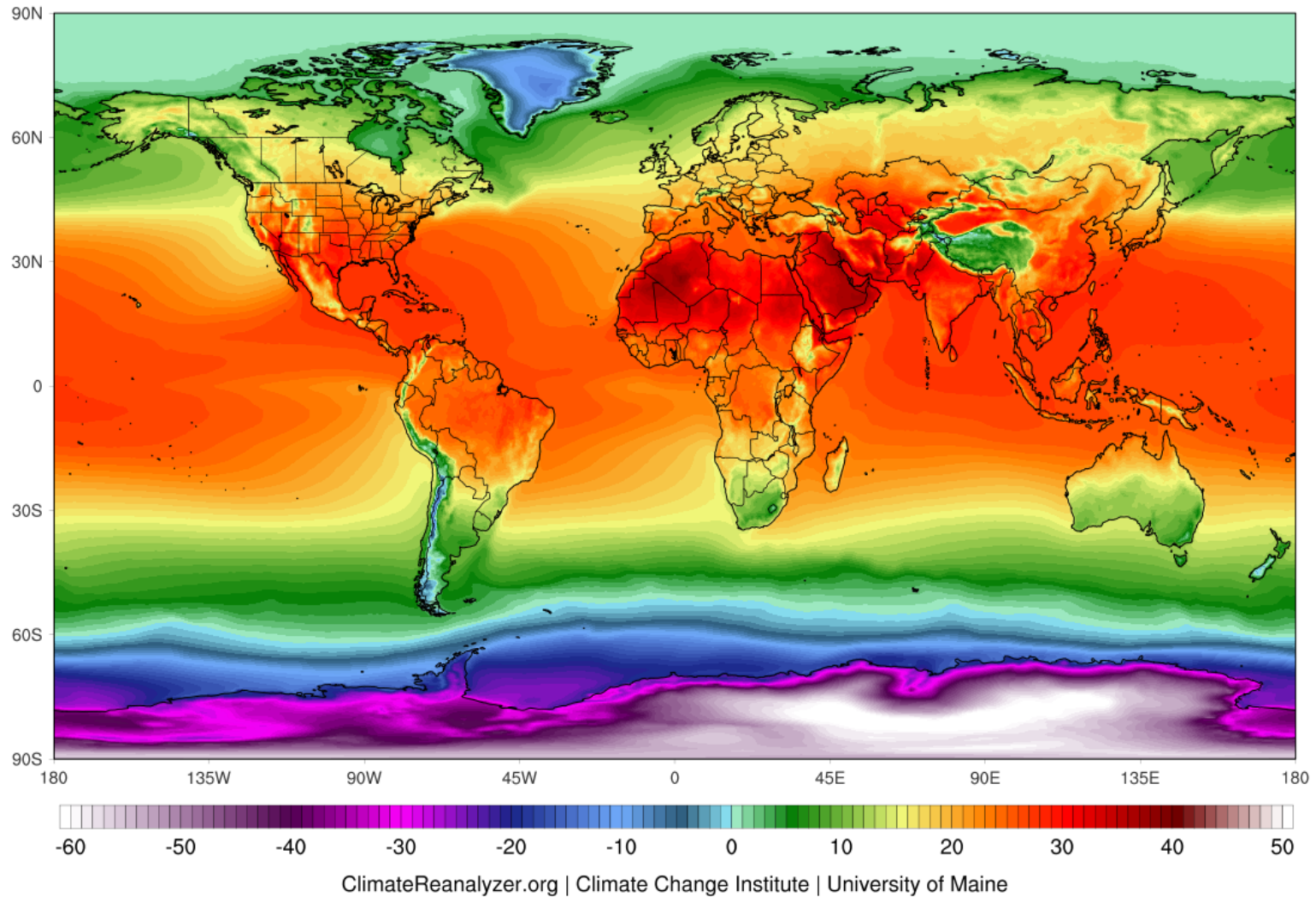
Figure 2.3. Average July air temperature at 2 meters above the Earth's surface, 1951-2020 (data – ECMWF European Reanalysis V5). Image Source: Courtesy of Climatoreanalyzer.org .
