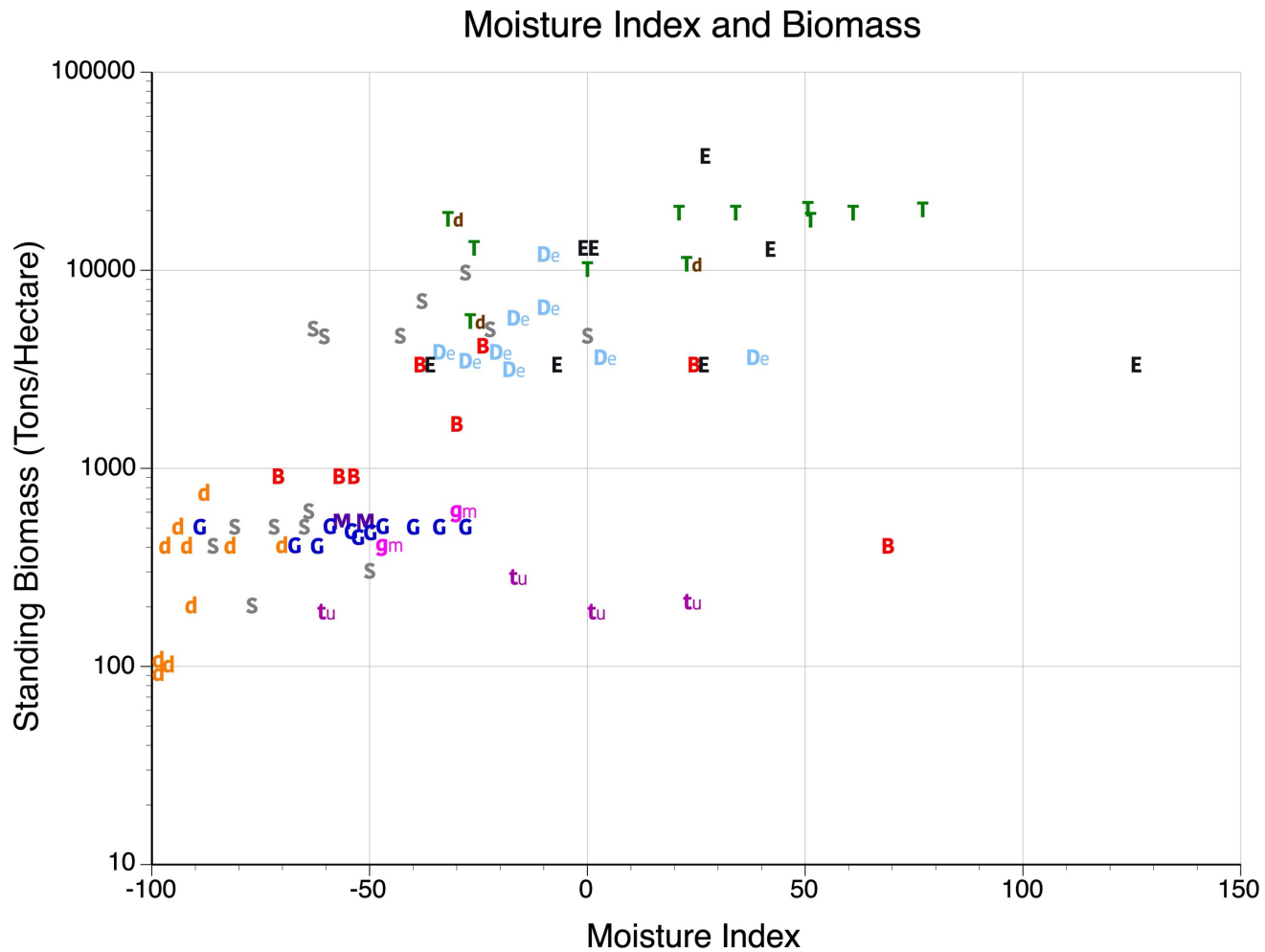
Figure 10.8. Relationship between measured standing biomass and moisture index for 80 sampled locations. Eleven types of biomes are shown: T = Tropical & Subtropical Moist Broadleaf Forests, Td = Tropical & Subtropical Dry Broadleaf Forests, S = Tropical & Subtropical Grasslands, Savannas & Shrublands, d = Deserts & Xeric Shrublands, gm = Montane Grasslands & Shrublands, M = Mediterranean Forests, Woodlands & Scrub, G = Temperate Grassland, Savannas & Shrublands, De = Temperate Broadleaf & Mixed Forests, E = Temperate Coniferous Forests, B = Boreal Forests, and tu = Tundra.
