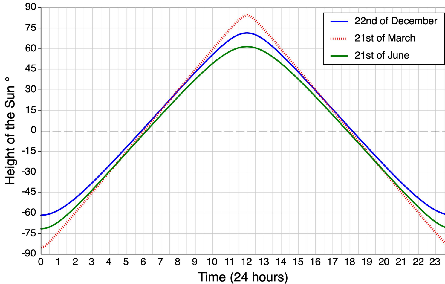
Figure 1.11. Height of the Sun above (+) or below (-) the horizon at different times during the day for December 22, March 21, and June 21 for a location found at 5° South. Image Copyright: Michael Pidwirny.
