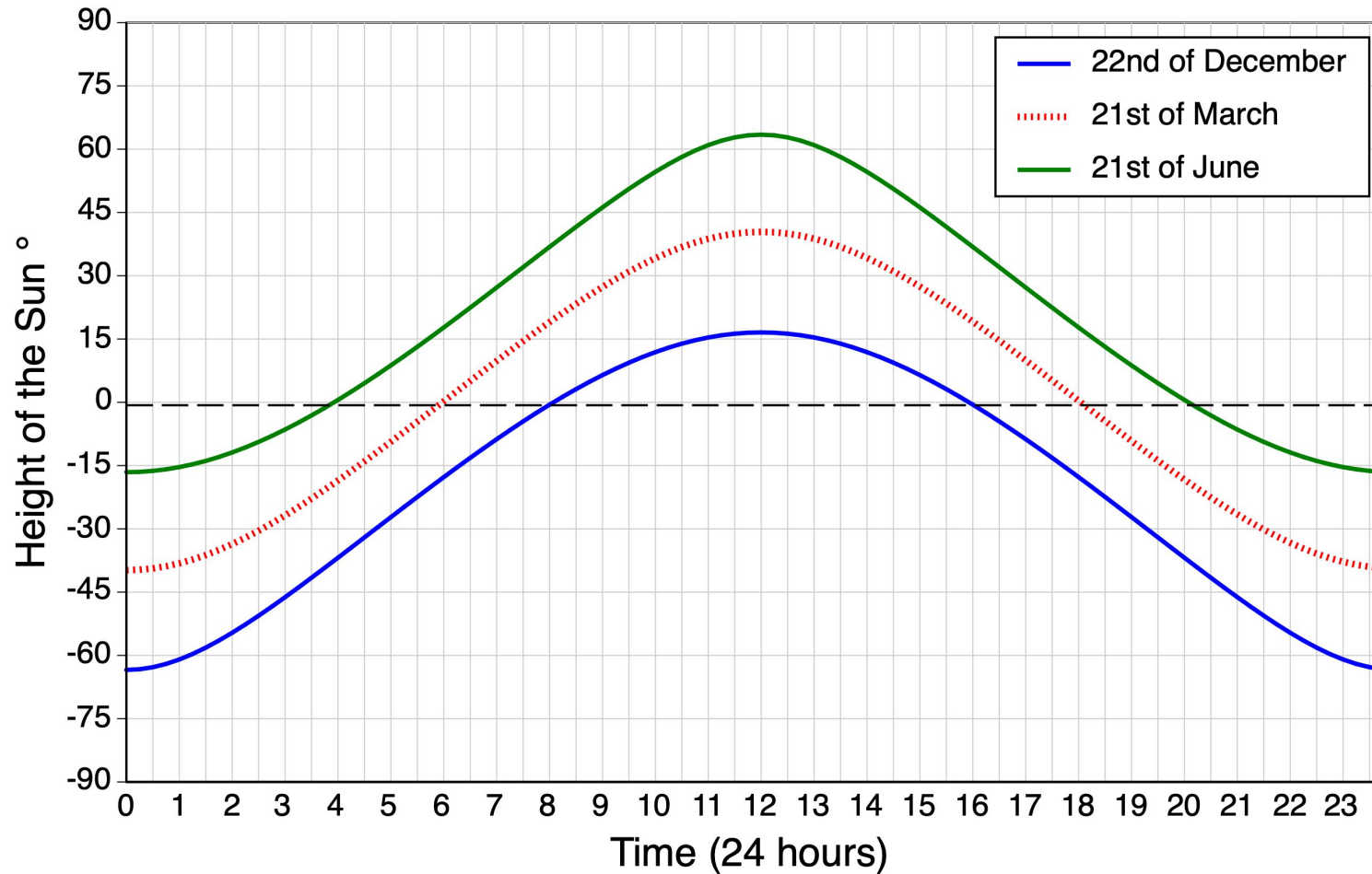
Figure 1.9. Height of the Sun above (+) or below (-) the horizon at different times during the day for December 22, March 21, and June 21 for a location found at 50° North. Image Copyright: Michael Pidwirny.
