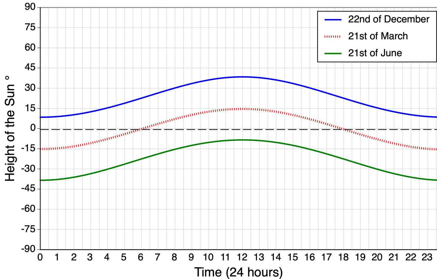
Figure 1.10. Height of the Sun above (+) or below (-) the horizon at different times during the day for December 22, March 21, and June 21 for a location found at 75° South. Image Copyright: Michael Pidwirny.
