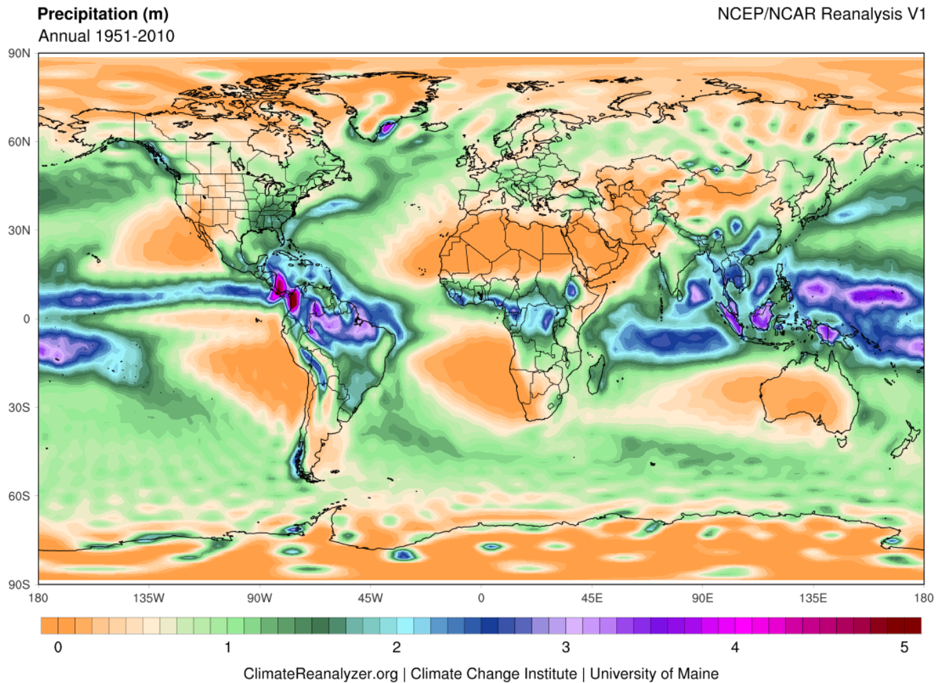
Figure 8.2. Average annual global precipitation in meters per year for the period 1951-2010. Image Source: Climate Reanalyzer, Monthly Reanalysis Maps . Data Source: NOAA National Center for Environmental Prediction, National Center for Atmospheric Research dataset version 1.
