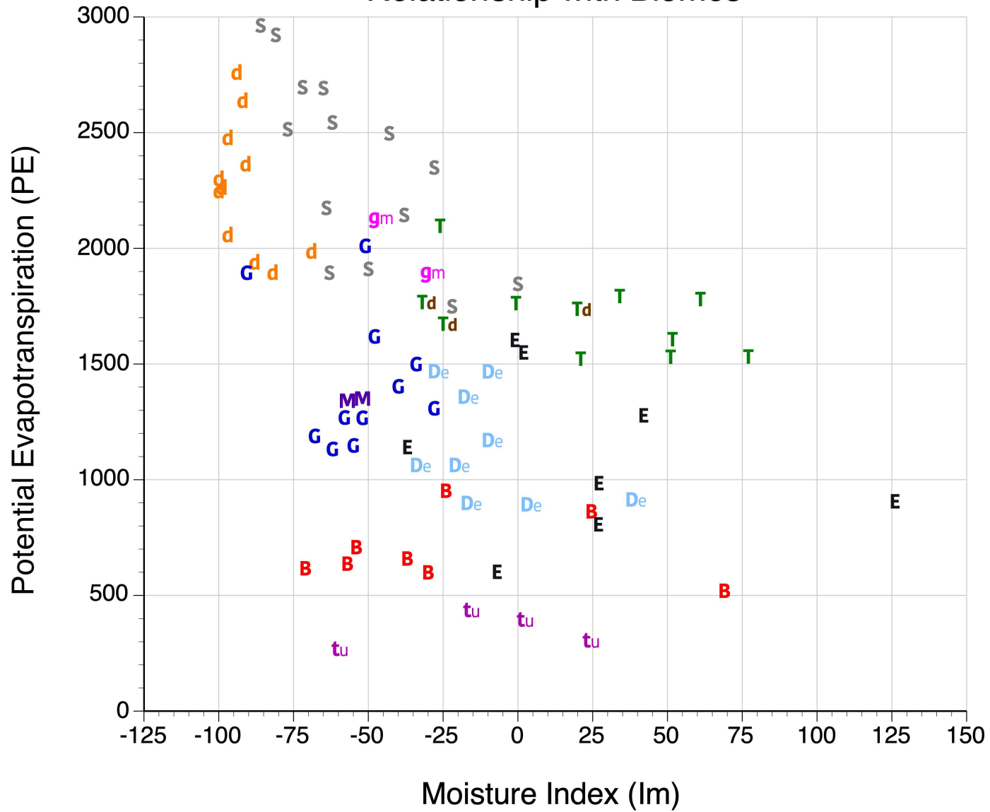
Figure 9.2. Plot of 80 locations with biome types, and measurements of potential evapotranspiration and moisture index.
