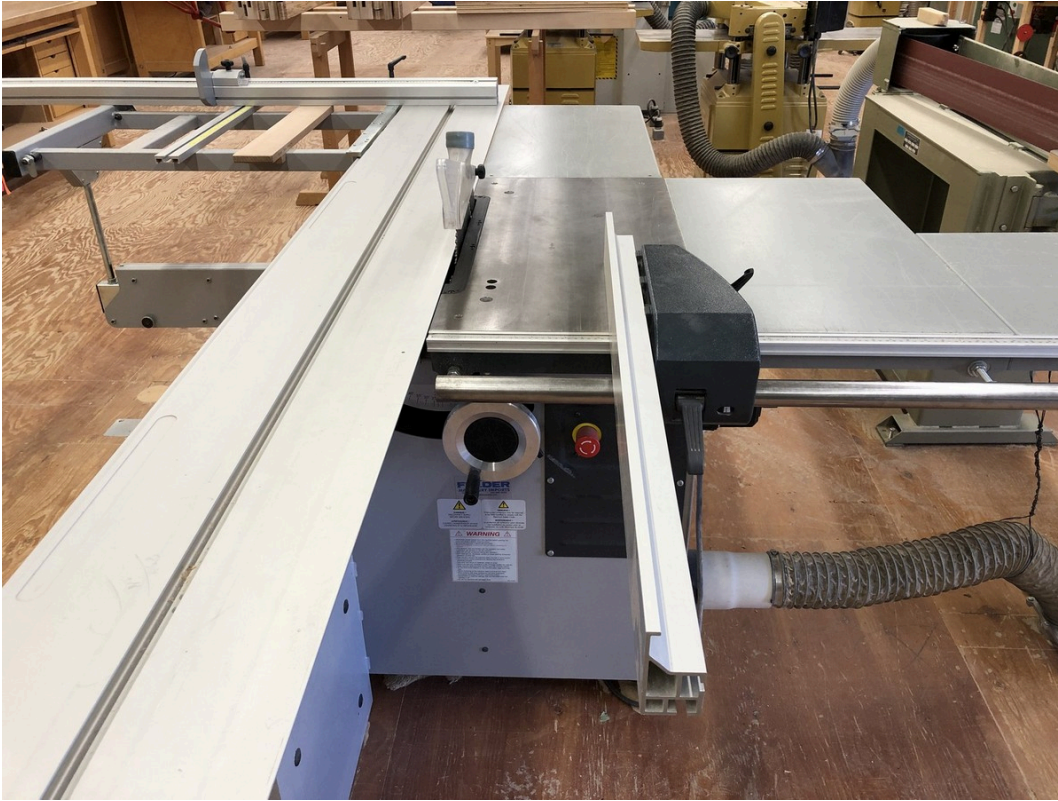
Rip fence positioned for use as a moveable stop for crosscutting.
